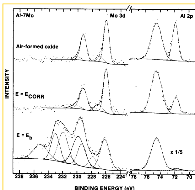
Fig. 7. The results of high-resolution XPS on the surface of an air-formed passive film, a passive film formed after exposure to the electrolyte at E_{CORR} , and a film at the breakdown potential, for both the Al 2p and Mo 3d peaks. The Al 2p state contains two peaks corresponding to the metallic (dashed) and the oxidized (dotted) states. On the other hand, Mo may contain up to four different valence states: metallic (dashed), Mo^{+3} (dotted), Mo^{+4} (long dashed), and Mo^{+5} (short dash-dot). Each state of Mo contains two peaks due to the doublet of the valence state. The size and shape of the second peak is dependent upon the height and area of the first peak.
