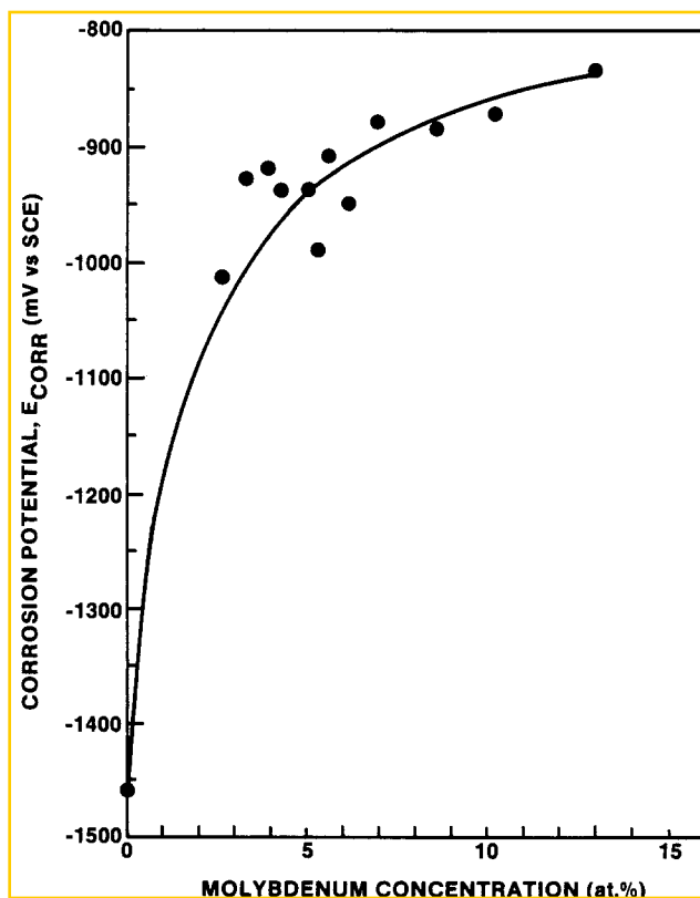
Fig. 5. The effect of the average Mo content in the alloy on the E_{CORR} .
