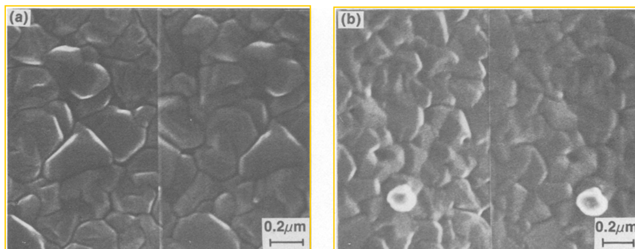
Fig. 2. Surface of a) pure Al and b) Al with 6 a/o Mo in solid solution after RF-magnetron sputter-deposition.
