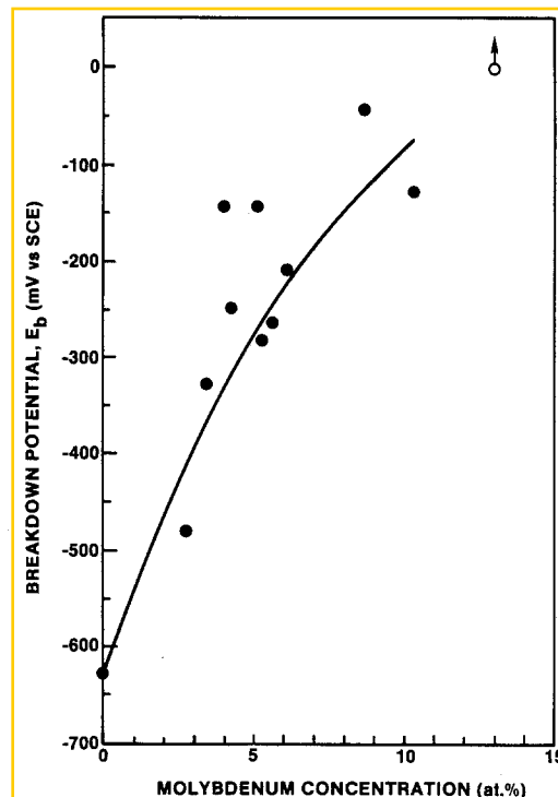
Fig. 6. The effect of the average Mo content in the alloy on the E_b , determined from a rapid increase in the current density during potential dynamic polarization.
