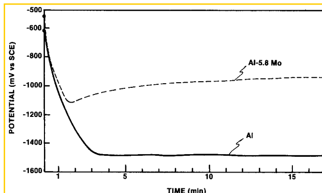
Fig. 4. The functional dependence of potential on the time of exposure of the working electrode to the 0.1N KCl electrolyte for pure Al and an Al-5.8 Mo alloy.
